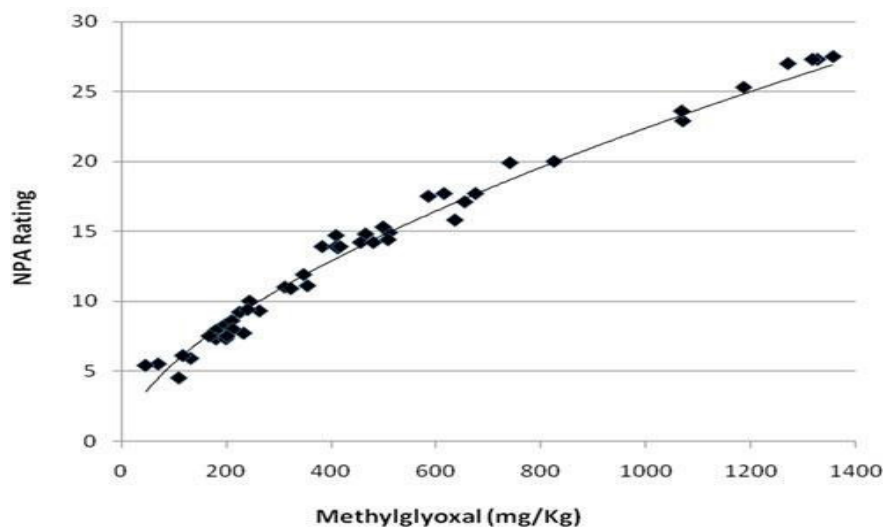
MGO to NPA conversion, from New Zealand honey data
